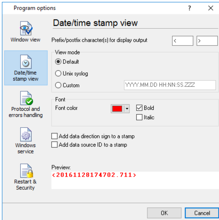
Fig. 29. Configuring data/stamp view
